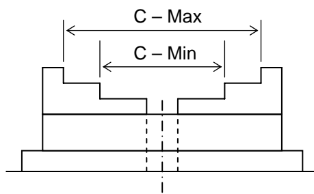
OUTSIDE CHUCKING
