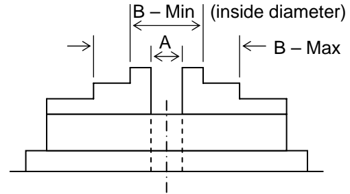
INSIDE CHUCKING
